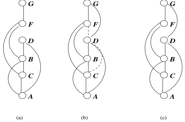
Figure 8: The induced augmented graph
