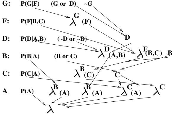
Figure 7: bucket elimination execution of elim-bel-cnfg
