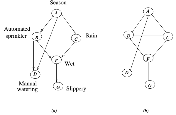
Figure 2: Belief network P(g, f, d, c, b, a) = P(g|f)P(f|c, b)P(d|b, a)P(b|a)P(c|a)P(a)
