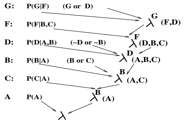
Figure 6: Bucket elimination execution of elim-CPE
