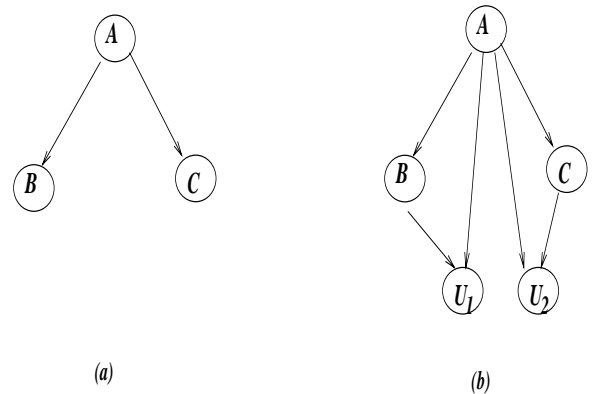
Figure 1: A three variable belief network (a), augmenting the query with a query subnetwork (b)
