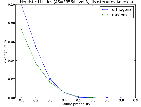
Fig. 5. The computed average utility metric of the two heuristics for various p(\text{fail}) values. Note the convergence of the curves on each other as p(\text{fail}) increases and fewer redundant paths are left undisrupted.
