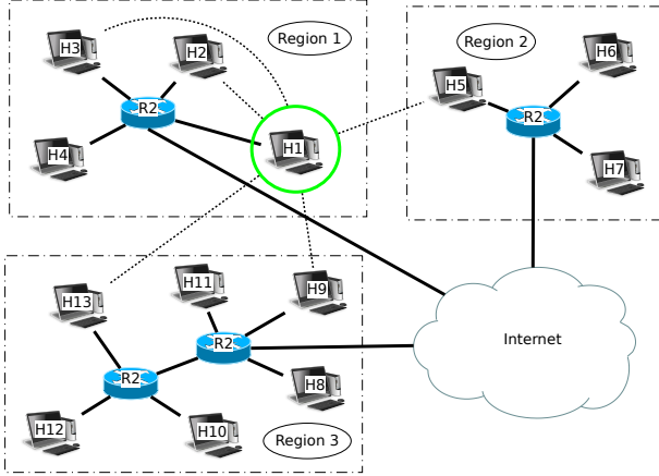
Fig. 2. A network overlay. The dashed edges incident with the circled node represent overlay connections. There are no direct physical connections between these nodes, but they can reach each other through their respective routers and the Internet with knowledge of each others' IP addresses.
