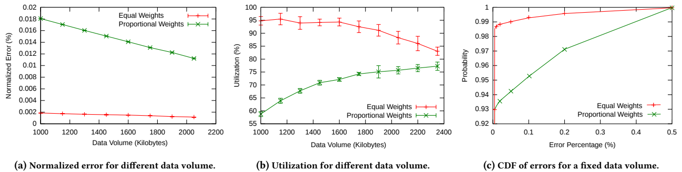
Figure 4: Different characteristics of adaptive sampling method.
