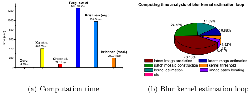
Fig. 5. Computation time analysis: (a) Computation time comparison between the algorithms. (b) The computation time analysis during the blur-kernel estimation loop.
