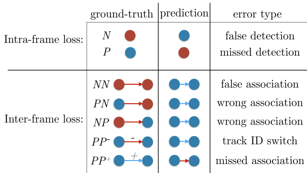
Fig. 4: Possible intra-frame and inter-frame errors a tracker could make which are penalized by our loss function. A blue node/edge indicates that corresponding flow variable is set to 1 in either ground-truth or tracker prediction. Similarly red node/edge indicates corresponding flow variable is set to 0.
