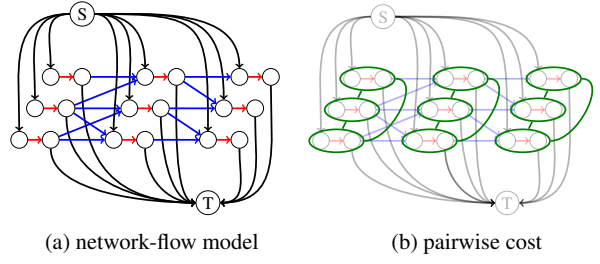
Fig. 2: Graphical representation of network flow model and its extension with pairwise costs. (a) Basic network-flow model for multi-target tracking, as described by Zhang et al (2008). A pair of nodes (connected by red edge) represent a detection, blue edges represent possible transitions between detections and track birth/death events are modeled by black edges. Costs c_i in Eq. 3 are for red edges, c_{ij} are for blue edges, c_i^t and c_i^s are for black edges. (b) Network-flow model extended with pairwise cost. A green node represents a detection site while an undirected edge between green nodes encodes the pairwise cost for choosing both detection sites as part of the solution. To simplify our description, in later text we will refer to a green node (a red edge and the two nodes associated with it) as a “detection node”. The set V consists of all detection nodes in the graph, whereas the set E consists of all transition edges in the graph.
