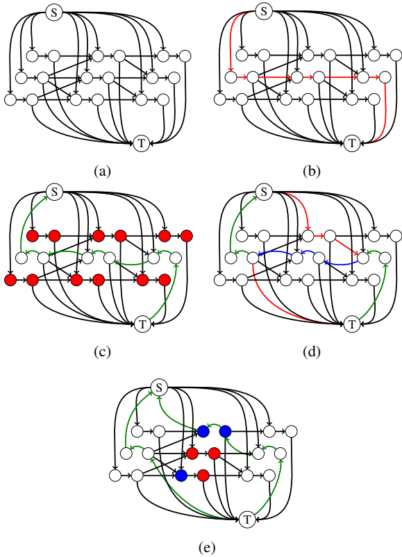
Fig. 3: An illustration for 2-pass DP with quadratic interactions. (a) the initial DAG graph, a pair of nodes indicate a candidate detection; (b) first iteration of the algorithm, red edges indicates the shortest path found in this iteration; (c) we reverse all the edges along the shortest path (green edges), and add the pairwise cost imposed by this path to other candidates detections at each time point (red node pairs). (d) In the second iteration of the algorithm, red edges and blue edges indicate the new shortest path which happens to traverse three of the reversed edges (shown in blue); (e) we again reverse all the edges along the shortest path yielding two instanced st-tracks (green edges). We again update pairwise cost: blue node pair indicates we subtract the pairwise cost imposed by “turning off” a candidate, red pair indicates adding in pairwise cost of newly instanced candidates, and the blue-red pair indicates we first add the pairwise cost by newly instanced candidates, then subtract the pairwise cost by newly uninstanced candidates. Additions and subtractions are done to the non-negated edge costs and then negated if necessary.
