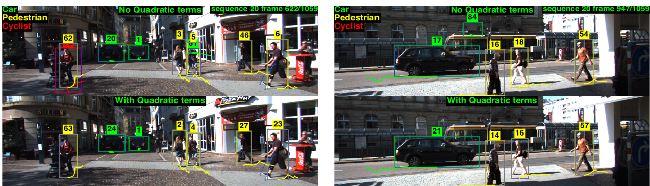
Fig. 8: Additional Qualitative Results on KITTI DPM detection set. The linear cost tracking model has wrongly labeled “a person pushing a cart” as “cyclist” (top-left), while our quadratic model is able to suppress cyclist trajectory with a high penalty between co-occurrence of pedestrian and cyclist (bottom-left). The quadratic interaction is also helpful in that it could help to suppress spatially infeasible co-occurrence from imperfect detectors, such as a car appearing on the back of a pedestrian (left), or a car “flying” above a pedestrian (right).
