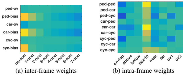
Fig. 5: Visualization of the weight vector learned on KITTI dataset for the DPM detector. Yellow has small cost, blue has large cost. (a) shows transition weights for different length of frame jumps. (b) shows learned pairwise contextual weights between objects. The model encourages intra-class co-occurrence when objects are close but penalizes overlap and objects on top of others. Note the strong negative interaction learned between cyclist and pedestrian (two classes which are easily confused by their respective detectors.). Figure is best viewed in color.
