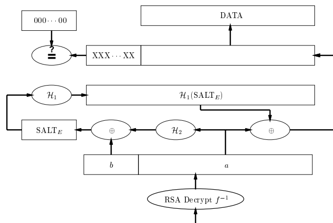
Fig. 14. Decryption using OAEP
