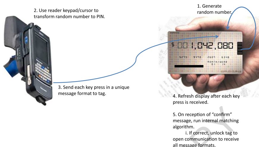
Fig. 2. Secure user-to-DERT authentication. (Colors are visible in the online version of the article; http://dx.doi.org/10.3233/JCS-130470 .)
