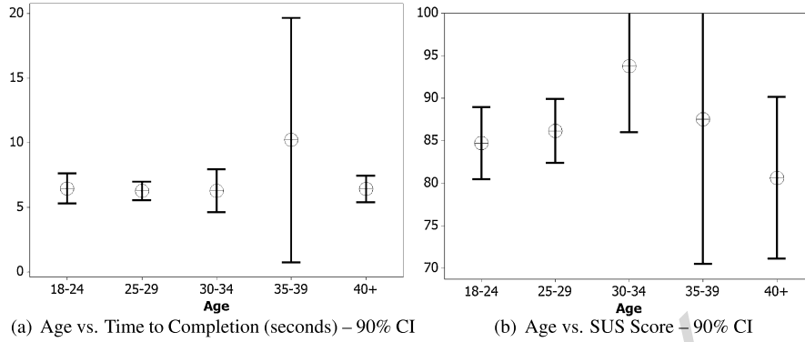
Fig. 6. Interval plots: performance of transaction verification protocol (crosshairs denote mean).
