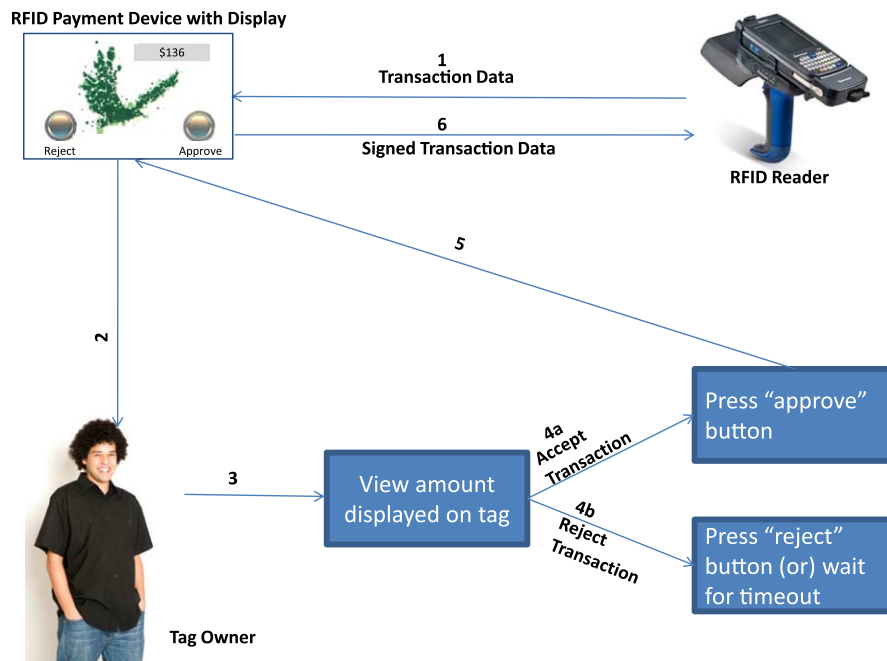
Fig. 3. DERT-enabled transaction verification. (Colors are visible in the online version of the article; http://dx.doi.org/10.3233/JCS-130470 .)
