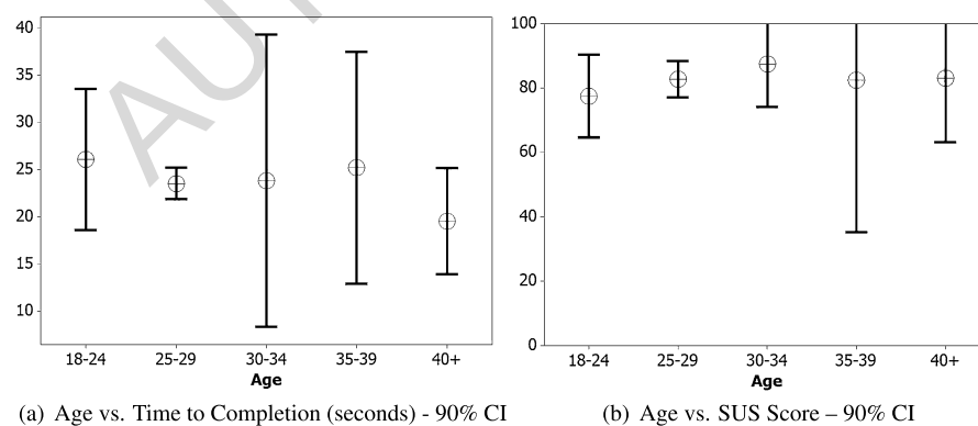
Fig. 8. Interval plots: performance of device pairing protocol (crosshairs denote mean).
