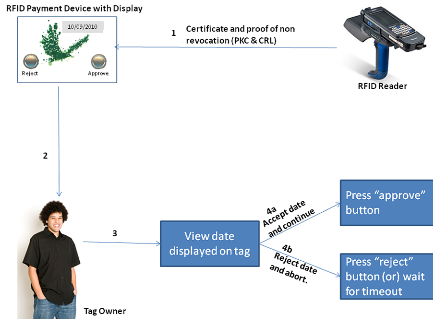
Fig. 4. Reader certificate expiration/revocation checking. (Colors are visible in the online version of the article; http://dx.doi.org/10.3233/JCS-130470 .)
