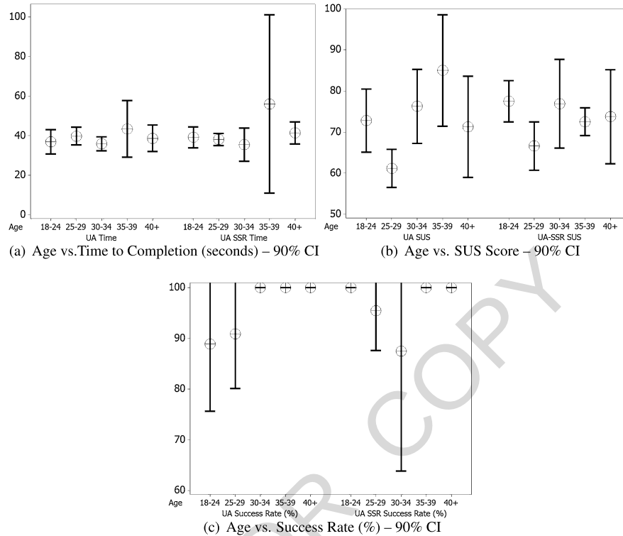
Fig. 5. Interval plots: performance of UA and UA-SSR variants (crosshairs denote mean).
