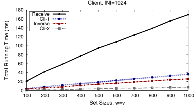
Figure 8: Micro-benchmarking client's operations in DT10-v4 (small sets), using 1024-bit moduli.
