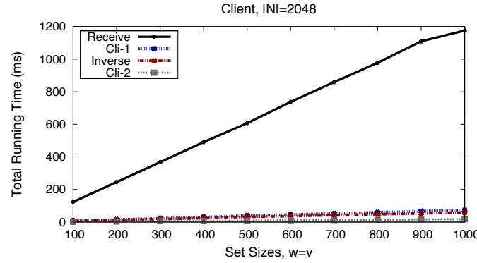
Figure 10: Micro-benchmarking client's operations in DT10-v4 (small sets), using 2048-bit moduli.
