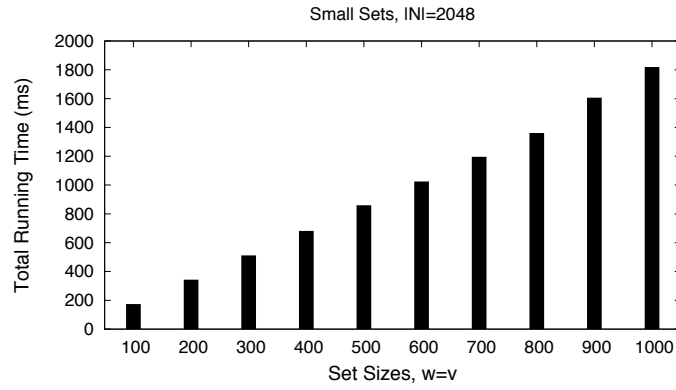
Figure 4: DT10-v4 total run-time for small sets (100 to 1000 items), using 2048-bit moduli.
