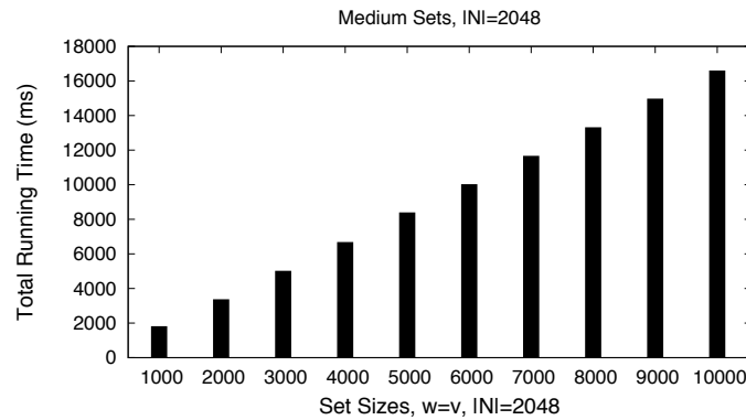
Figure 5: DT10-v4 total run-time for medium sets (1000 to 10000 items), using 2048-bit moduli.
