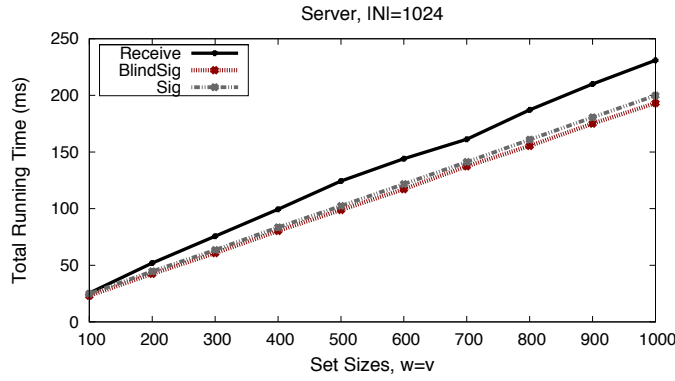
Figure 9: Micro-benchmarking server's operations in DT10-v4 (small sets), using 1024-bit moduli.
