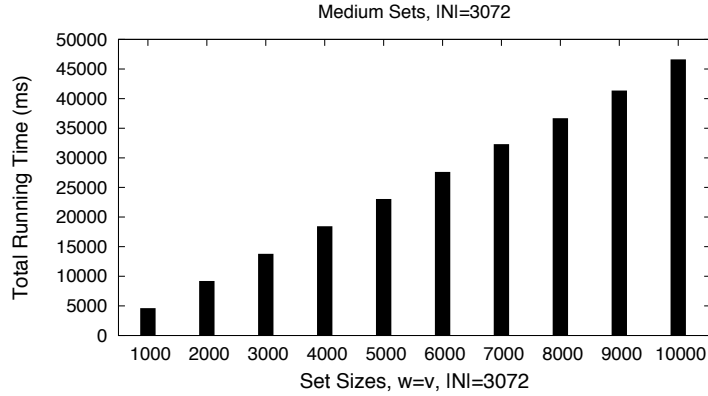
Figure 7: DT10-v4 total run-time for medium sets (1000 to 10000 items), using 3072-bit moduli.
