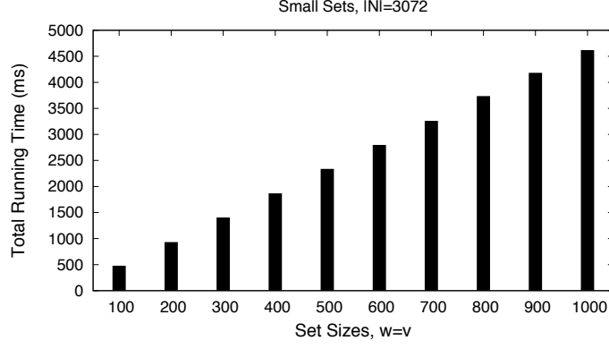
Figure 6: DT10-v4 total run-time for small sets (100 to 1000 items), using 3072-bit moduli.
