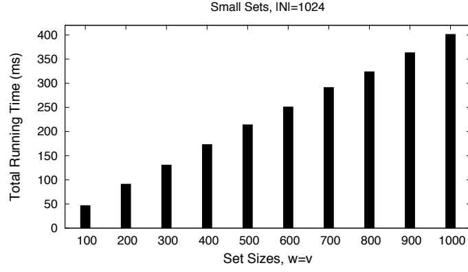
Figure 2: DT10-v4 total run-time for small sets (100 to 1000 items), using 1024-bit moduli.
