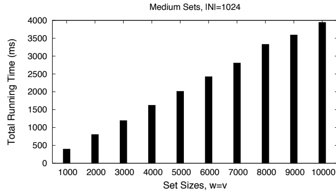
Figure 3: DT10-v4 total run-time for medium sets (1000 to 10000 items), using 1024-bit moduli.
