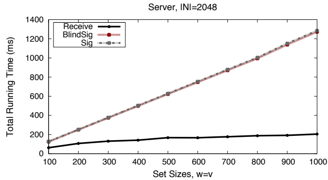
Figure 11: Micro-benchmarking server's operations in DT10-v4 (small sets), using 2048-bit moduli.
