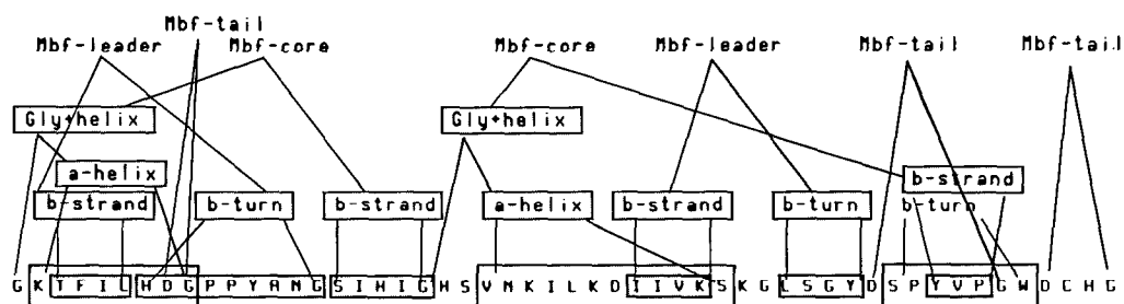
FIGURE 4d. E. coli Ile-RS (residues 48-99 of 939 residues) (Intermediate predictions constructed by ARIADNE)
