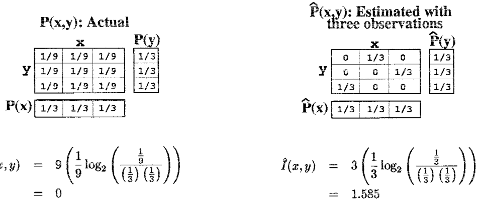
Fig. 1. This figure illustrates why mutual information is overestimated with small sample sizes. Left: The actual probability distribution of random variables X and Y , with a mutual information of zero. Right: The probability distribution computed with three observations, yielding an observed mutual information of 1.585 bits.
