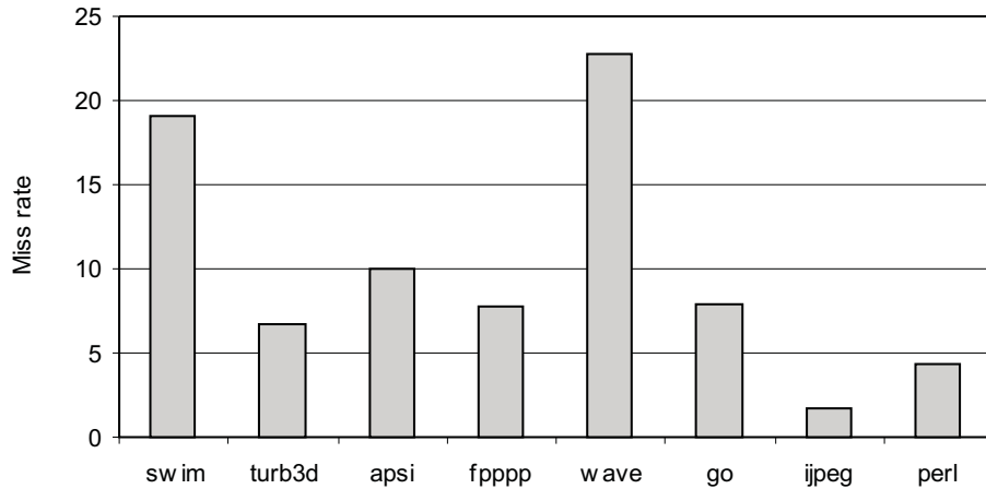
Fig. 2. L1 miss rate of 16KB direct-mapped, 32B line size cache
