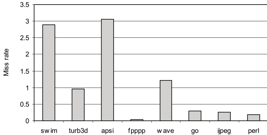
Fig. 3. L2 miss rate of 256KB, 2-way set associative, 64B line size L2 cache
