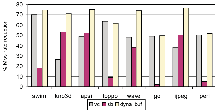
Fig. 9. Miss rate reduction for dyna_buf.
