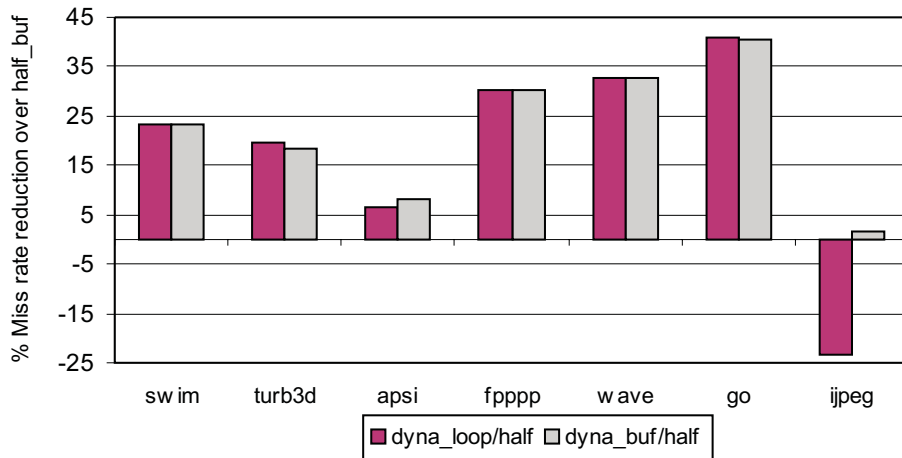
Fig. 12. Dyna_loop and dyna_buf performance relative to half_buf for a 256B cache assist.
