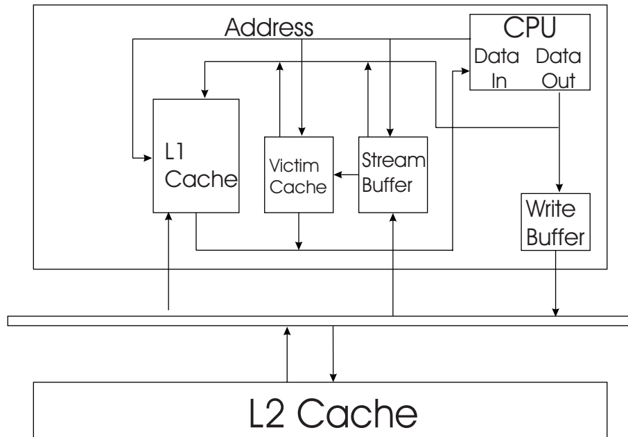
Fig. 1. System design
