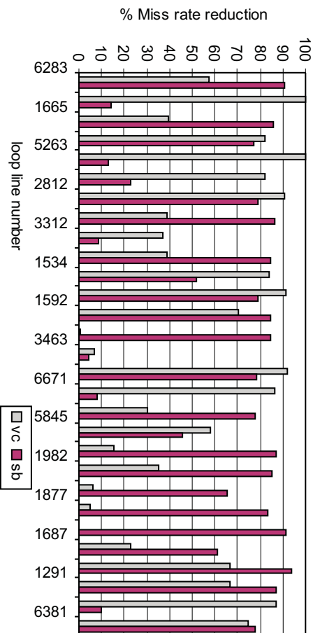
Fig. 5. Miss rate reduction per loop (a 1KB assist, the apsi benchmark)
