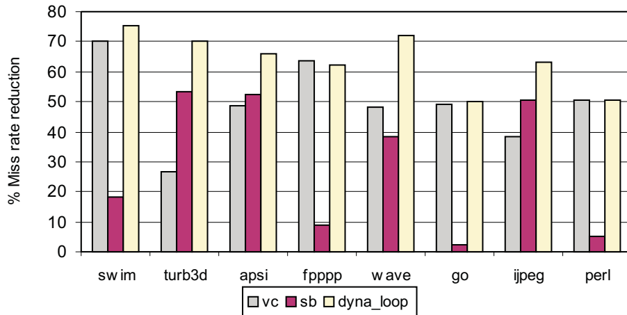
Fig. 7. Miss rate reduction for dyna_loop .
