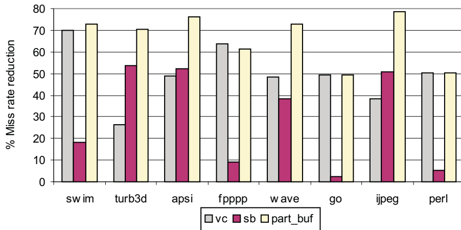
Fig. 8. Miss rate reduction for part_buf.
