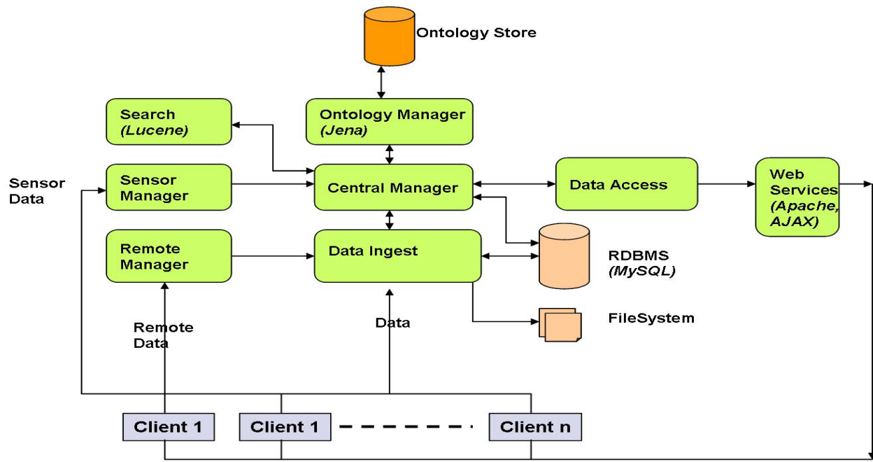
Fig 2 EBox System Architecture
