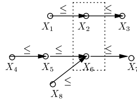
Figure 3: An inequality graph G(v) .
