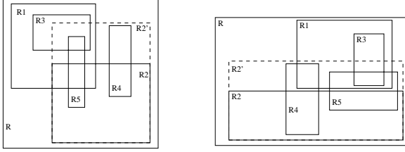
Figure 2: Insertions cause leaf granules to grow into other tree granules. (a) shows the problem with the cover-for-insert and overlap-for-search policy (b) shows the problem with overlap-for-insert and cover-for-search policy.
