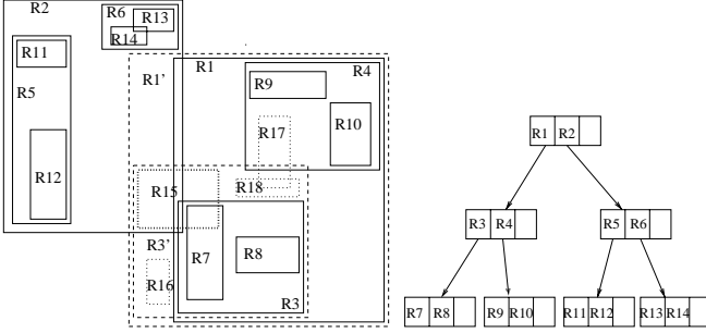
Figure 3: Insertions cause external granules to shrink. R15 is the object being inserted. R16 , R17 and R18 are other predicate rectangles. The R-tree corresponding to the initial spatial distribution of the objects is shown alongside.
