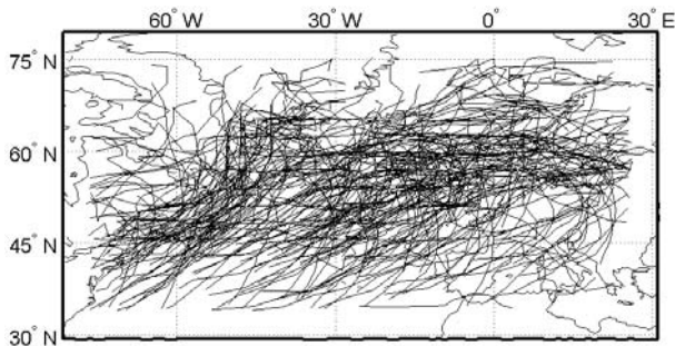
Figure 7: A subset of the North Atlantic cyclone trajectory data.
