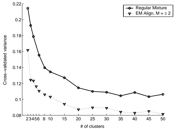
Figure 3: Within-cluster mean variance (out-of-sample) for methods with and without time-shifts on gene expression data.
