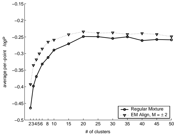
Figure 4: Cross-validated logP scores on gene expression data with V = 10 .
