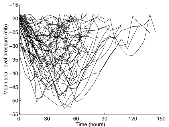
Figure 1: Curves of cyclone intensities from genesis to death.
