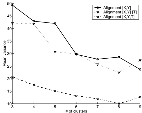
Figure 9: Average within-cluster variance on cyclone data.
