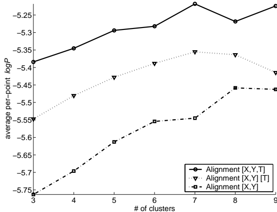
Figure 8: Cross-validated logP scores on cyclone data.
