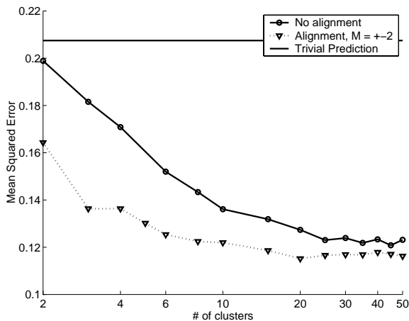
Figure 5: Cross-validated MSE of one-step-ahead prediction on gene expression data.
