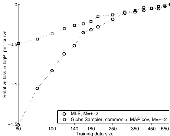
Figure 6: Average improvement in out-of-sample logP scores for various training sample sizes using Bayesian estimation on gene expression data with K=10 .
