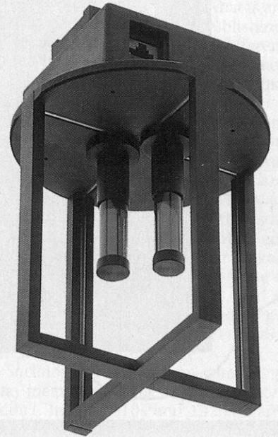
RADIO TRANSCEIVER links pads and other movable computer devices to the wired network. This unit, intended to be mounted on the ceiling, contains antennas in its crossed arms and two light-emitting diodes to signal its status.
