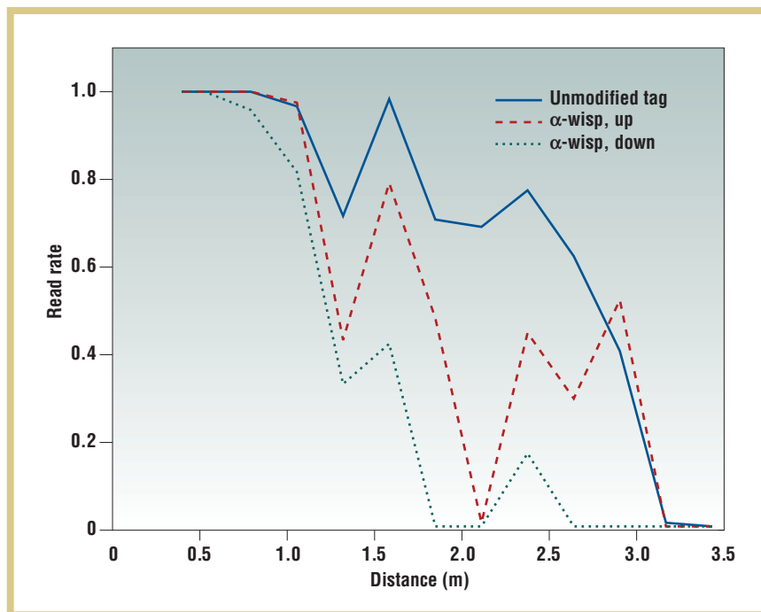
Figure 2. The dependence of read rate on read distance. Data is for an \alpha -wisp serial-switch configuration. Read rate is the fraction of reads in which the reader detected a single stationary tag with no occlusion in typical indoor conditions. \alpha -wisps are detectable beyond 3.0 meters from the reader. Read rates are lower than for unmodified RFID tags.
