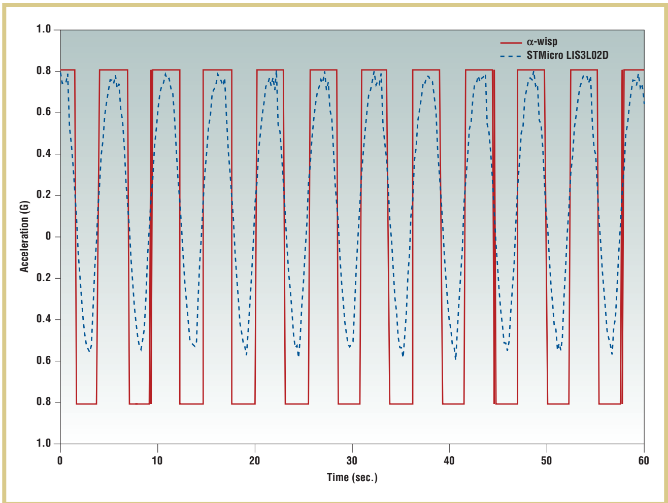
Figure 4. An \alpha -wisp parasitically powered one-bit accelerometer in operation. Comparison of data returned by the \alpha -wisp (the red trace) with continuous acceleration data provided by an STMicroelectronics LIS3L02D accelerometer (the blue trace).
