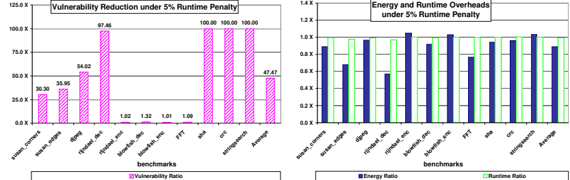
(a) Vulnerability Reduction (A bar greater than 1.0× indicates vulnerability reduction) (b) Energy and Runtime Increase (A bar lower than 1.0× indicates the overhead)
