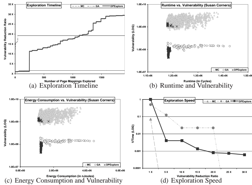
Fig. 7 Exploration by MC, GA and DPEXplore: DPEXplore effectively explores the design space
