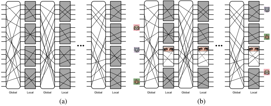
Fig. 1. (a) A parallel mixnet with n = 16 inputs and M = 4 mix servers. Shaded boxes illustrate mix servers, whose internal permutations are hidden from the adversary. The adversary is allowed to see the global permutation performed in each round. (b) A corrupted parallel mixnet, where s = 3 servers are not colluding with the adversary, who has injected f = 3 fake messages into the network.
