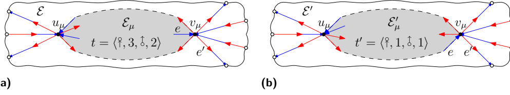
■ Figure 4 Illustration for the proof of Lemma 10. The parity of t and t' is the same at u_\mu and different at v_\mu ; in particular, even if a new alternation is introduced between the pair (e, e') at v_\mu , the different parity guarantees that the modality at v_\mu does not increase from \mathcal{E} to \mathcal{E}' .
