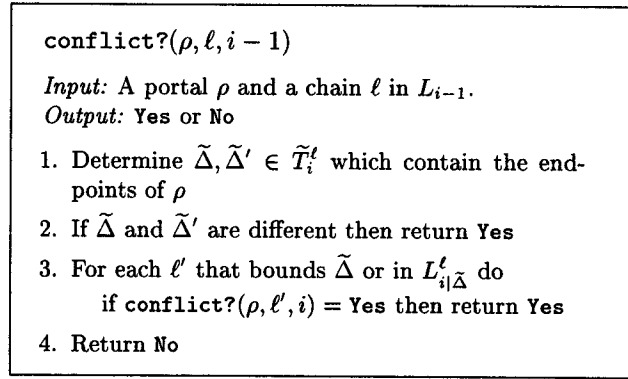
Figure 12: Portal-chain query procedure.
