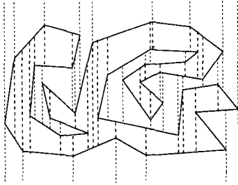
Figure 2: The trapezoidation of a simple polygon.
