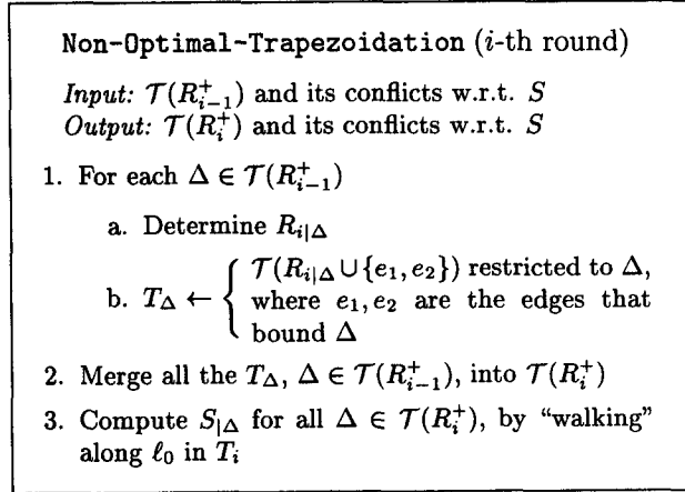
Figure 3: Non-optimal trapezoidation procedure.
