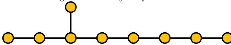
Figure 5: A graph Y whose Laplacian eigenvectors are uncomputable by a radical tree.
