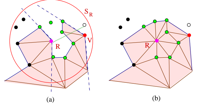
Figure 1: (a) Visibility test around R . The black points are behind R ’s boundary edges, the white points are occluded by other edges, and the point V is eliminated as R is behind its boundary edges. (b) Completed mesh at R
