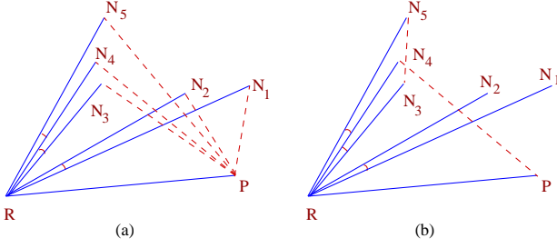
Figure 3: Pruning by Angle Criterion: (a) Ordering around R and P ; angles between N_1N_2 , N_3N_4 , and N_4N_5 are less than \beta . (b) N_3 trapped in \triangle RPN_4 , and N_4 trapped inside \triangle RN_3N_5
