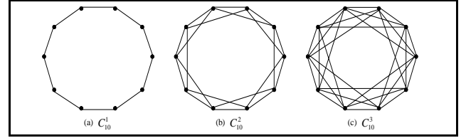
Figure 6: Examples of the T -th power of a circle.
