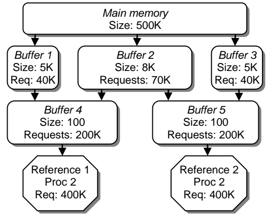
Figure 3. Example of a multiprocessor data reuse graph.
