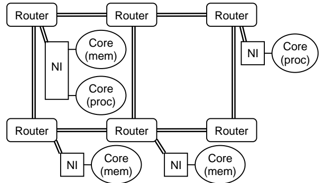
Figure 1. Example of 3x2 mesh-type NoC communication architecture.
