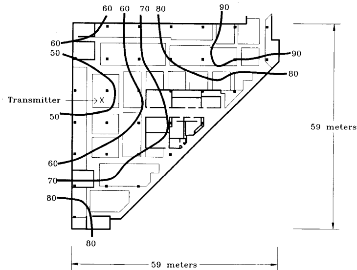
Fig. 8. Contour plot of locations with equal path loss in 10 dB steps for the fourth floor of the West wing of office building 1. The transmitter was located on the left side of the figure.
