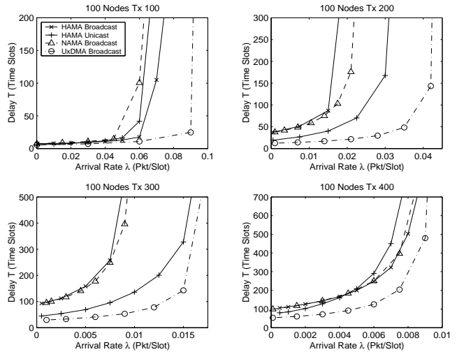
Figure 12. Average packet delays in multihop networks
