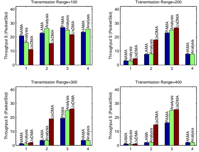
Figure 11. Packet throughput in multihop networks
