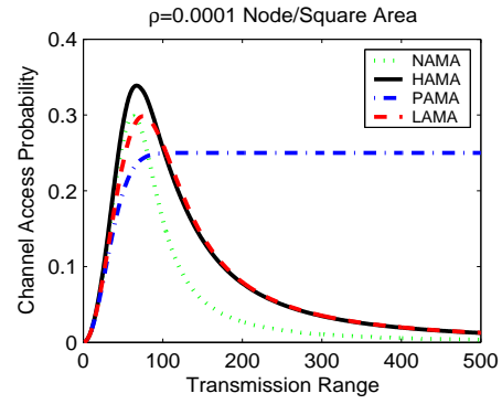
Figure 6. Channel access probability of NAMA, HAMA, PAMA and LAMA.
