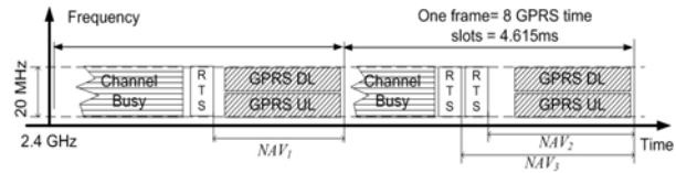
Figure 4 GPRS and WiFi time sharing the ISM spectrum.
