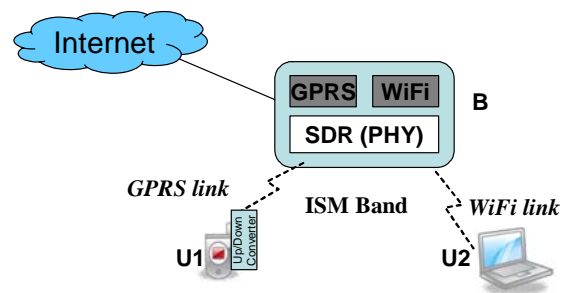
Figure 1 A base station supports both GPRS (with frequency converter) and WiFi units over the common ISM carrier.
