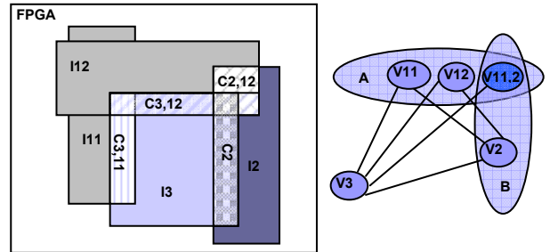
Fig 5. Parallel implementation for tasks T1 and T2 in graph representation.
