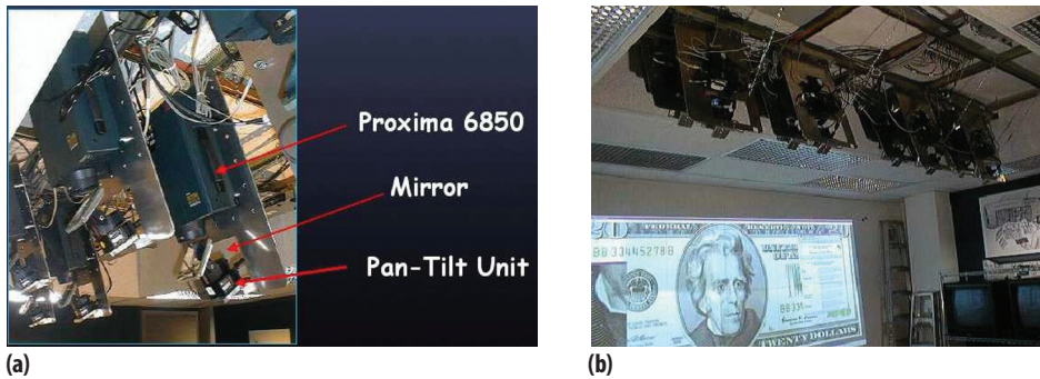
Figure 3. Evolution of automatic registration techniques. (a) Automatic panning and tilting in UNC's Pixel Flex project and (b) a PTU-mounted mirror that directed each projector's light to different areas of the flat wall, enabling the display to operate in a different scale, form factor, and aspect ratio. Although these systems are no longer operating, their design inspired a new generation of systems that use automatic registration.
