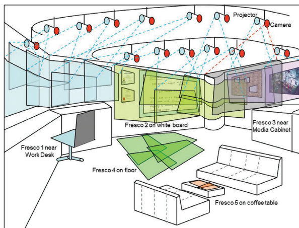
Figure 7. How ubiquitous displays might work. Active displays created by augmenting a projector with sensors (including a camera) and a computation and communication unit form a distributed network, or fresco , that users can move and reconfigure as needed.
