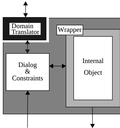
Figure 2-2. The Internal Architecture of a C2 Component.
