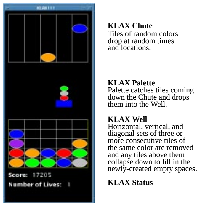
Figure 2-4. A snapshot and description of our implementation of the KLAX™ video game.
