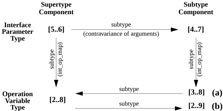
Figure 4-6. Relationship between supertype's and subtype's operation variable types. Contravariance of arguments and the int_op_map function do not guarantee a particular relationship between supertype's and subtype's operation variable types (illustrated using integer subranges): (a) supertype component's variable type is a supertype of subtype component's; (b) supertype component's variable type is a subtype of subtype component's.
