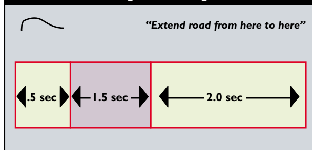
Figure 3. A sequentially integrated multimodal command, with pen input preceding speech and a brief lag between signals.
