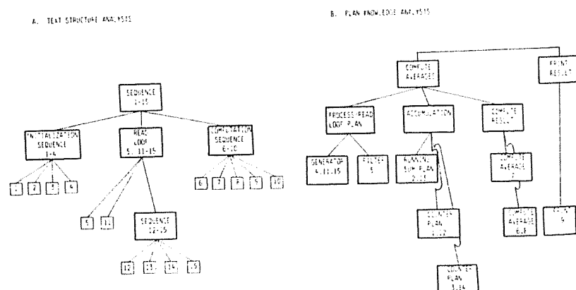
FIG. 6. Example analyses of the program segment shown in Fig. 1A. (Numbers refer to statement numbers in Fig. 1A.)
