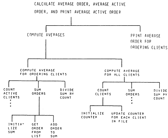
FIG. 2. Abstraction of function: The program accomplishes certain goals by producing outputs. Each level indicates a higher order goal that is decomposed into subgoals.
