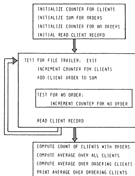
FIG. 4. Abstraction of control flow: Program actions occur in a particular sequence.
