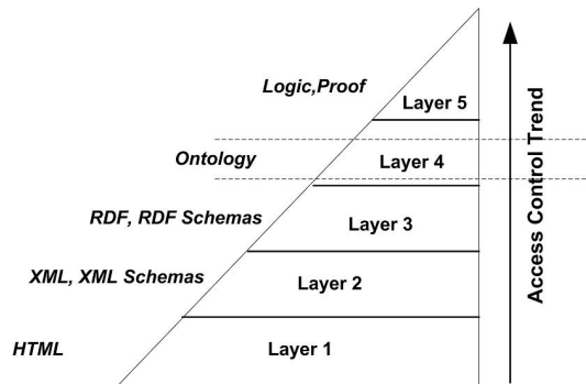
Fig. 1. SBAC in the Stack of Semantic Web
