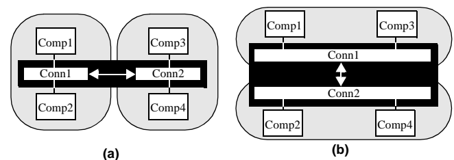
Figure 4. Connectors are a primary vehicle for distribution and heterogeneity. A single conceptual connector can be "broken up" (a) vertically or (b) horizontally for this purpose. Shaded ovals represent language, process, and/or machine boundaries.
