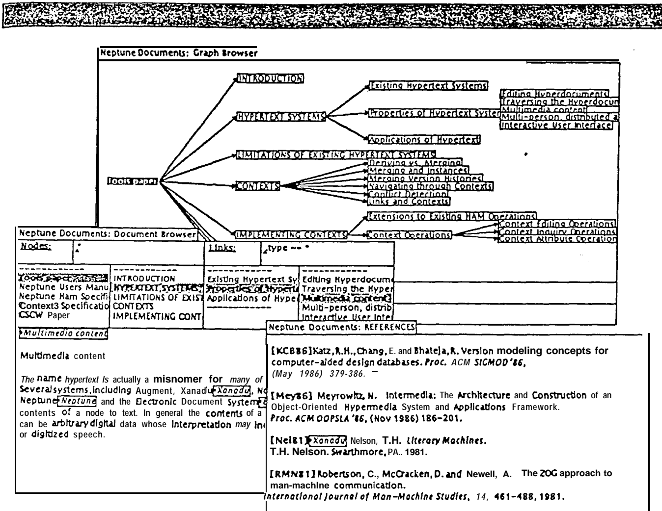
Figure 9. Neptune browsers. Three browsers from Neptune are illustrated. A pictorial view of a network of nodes and links is shown in the Graph Browser (the upper window). The lower right window and the lower pane of the Document Browser are viewers for text nodes. Icons representing link attachments are shown embedded within the text in each of the nodes.
