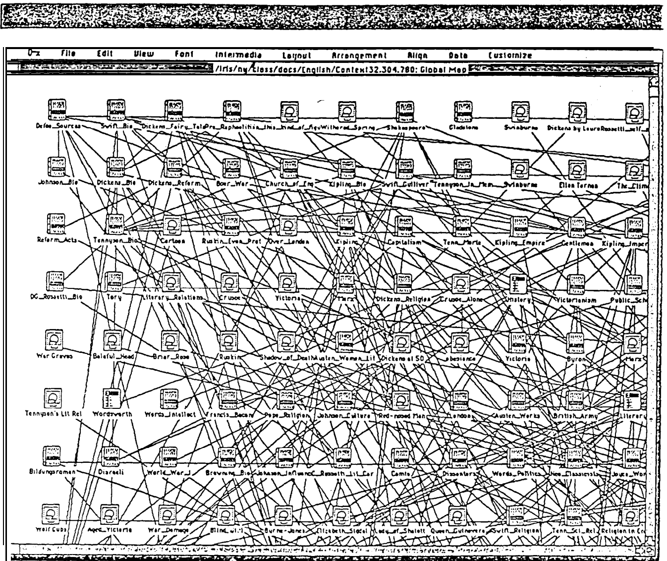
Figure 11. Tangled web of links. This experimental implementation of a global map in the Intermedia system shows the difficulty of providing users with spatial cues once a linked corpus contains more than a few dozen documents. This global map only represents about one tenth of the documents in a corpus designed for a survey of English literature course.
