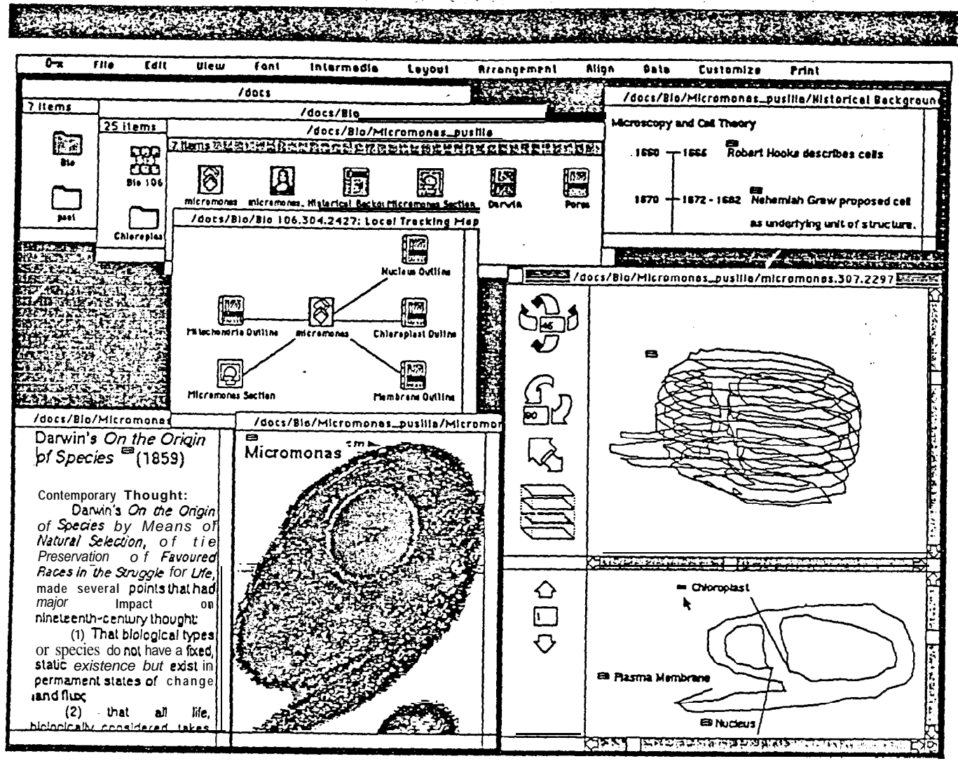
Figure 8. The Intermedia System. This figure illustrates materials from an Infermedia corpus called "Bio 106: Cell Biology in Context." Three folder windows containing hierarchically organized documents of different types are open in the upper left side of the display. An InterText document (lower left side) and an InterVal document (upper right side) are currently open, as well as an InterDraw document containing a scanned electronmicrograph (lower middle). This image has been linked to a corresponding three-dimensional image displayed in an InterSpect document (lower right). The "lower tracking map" (center) shows the link emanating from the current document. Authors or browsers can manipulate the three-dimensional image, edit text and graphics, follow links or create links at any time in this environment. (The electronmicrograph of Micromonas was published in the Journal of Phycology and is reprinted with the permission of the Editor.)
