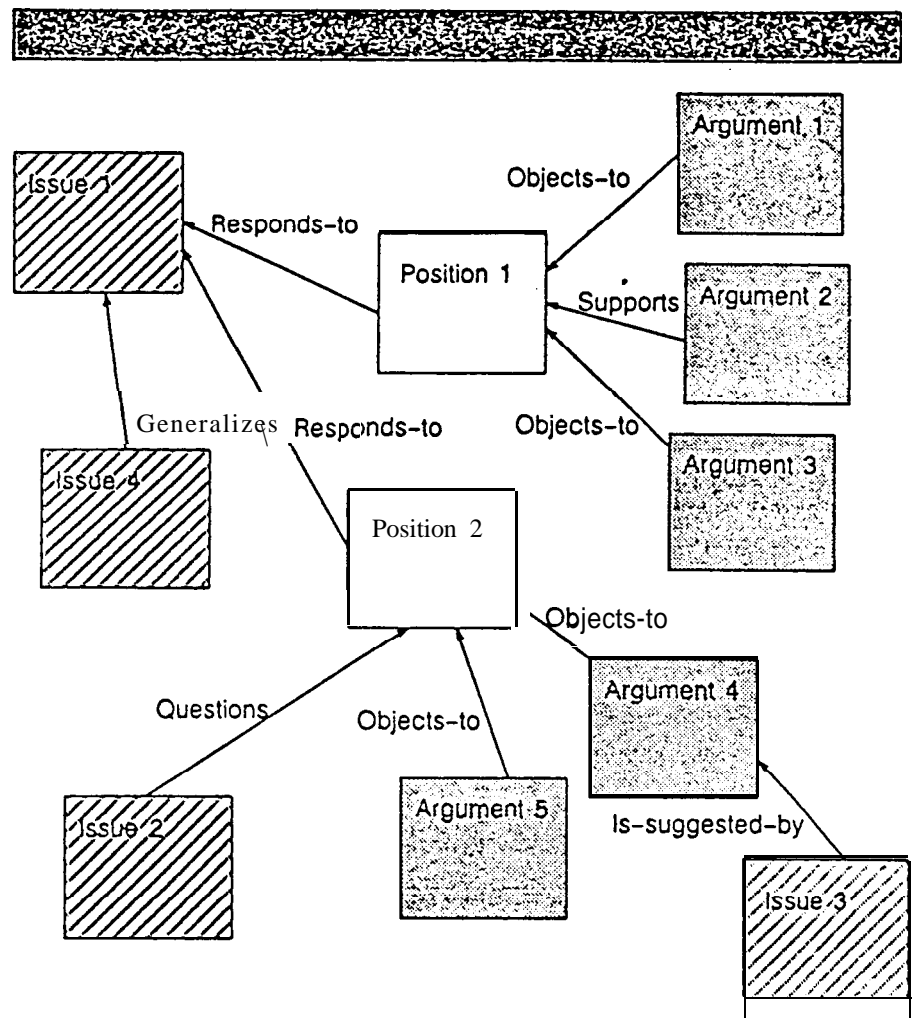
Figure 5. A segment of a possible IBIS-style discussion showing the topology of the IBIS network. Each node contains information on the type of the node, the time and date of creation, the author, a short phrase describing the content, a longer body of text with the text of the comment, a list of keywords, and a list of the incoming and outgoing links.
