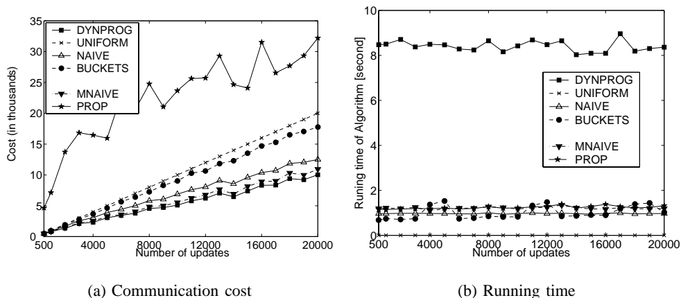
Fig. 8. Effect of query weights on communication cost. ( \mathcal{M}_2 ; 6,000 queries; query-length distribution: G(500, 400) .)
