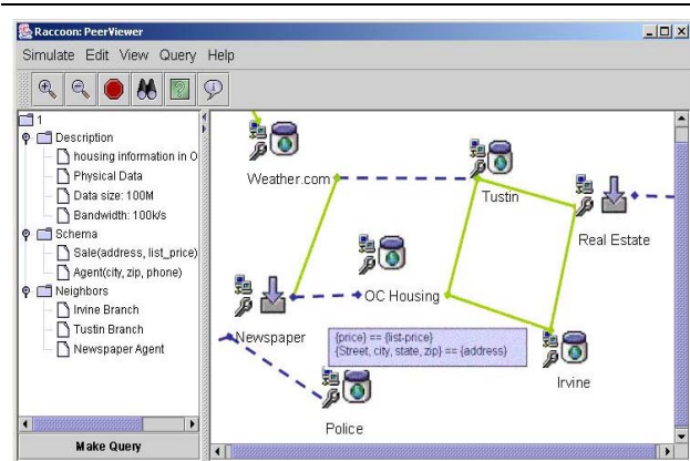
Figure 1. PeerViewer.
