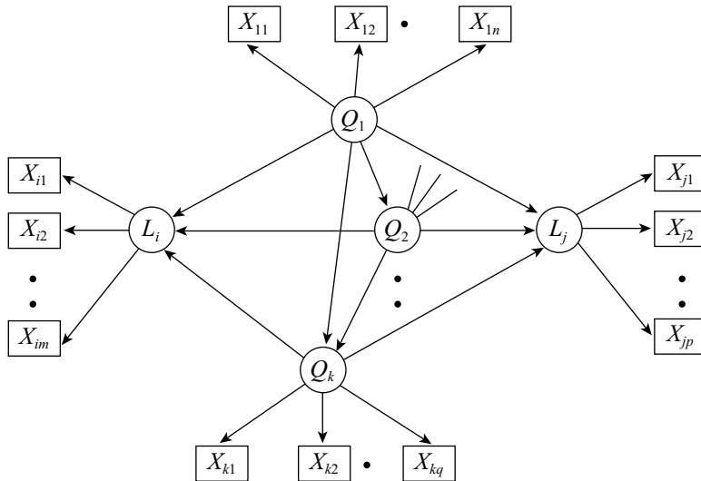
Figure 12.18. Model M_0 for testing L_i \perp\!\!\!\perp L_j \mid \mathbf{Q} .
