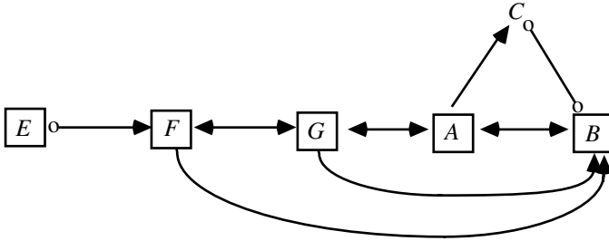
Figure 13.3. \langle E, F, G, A, C, B \rangle is a definite discriminating path for C
