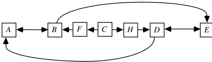
Inducing Path Graph G
