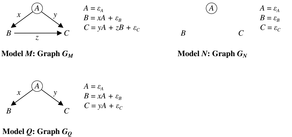
Figure 12.11. Model M , Model N , and Model Q
