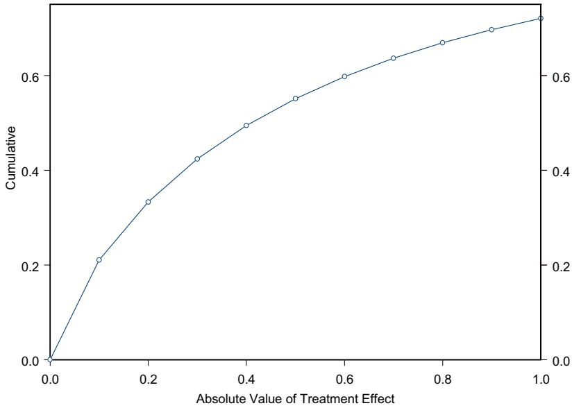
Figure 12.14. Cumulative distribution over |z| conditional on \rho(B,C) = 0
