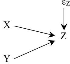
Figure 2. DAG illustrating direct effect modification of the effect of Y on Z in X
