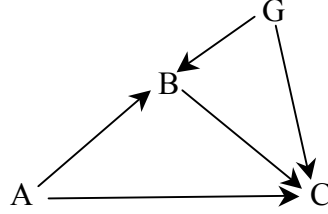
Figure 3. DAG consistent with effect modification of the effects of A on B, and B on C and/or A on C, in G
