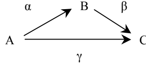
Figure 1. A simple linear path model
