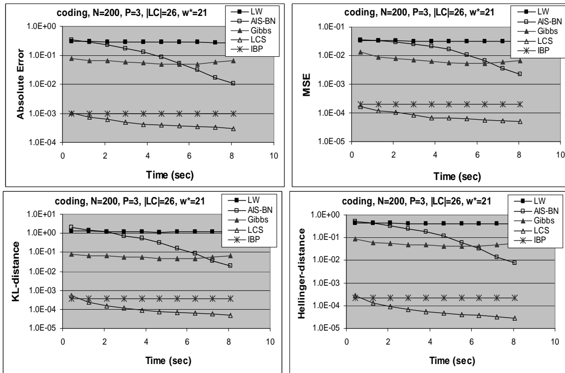
Figure 13: Comparing loop-cutset sampling (LCS), w_{LC}=3 , Gibbs sampling (Gibbs), likelihood weighting (LW), AIS-BN, and IBP on coding networks, \sigma=0.4 , averaged over 10 instances of 10 coding networks (100 instances total). The graphs show average absolute error ( top left), MSE (top right), KL-distance (bottom left), and squared Hellinger’s distance (bottom right) as a function of time.
