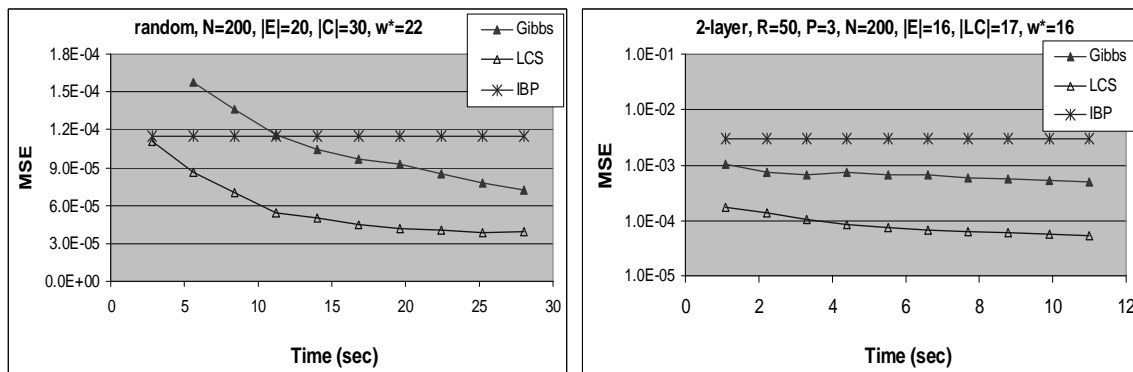
Figure 14: Comparing loop-cutset sampling (LCS), Gibbs sampling (Gibbs), and IBP on random networks (left) and 2-layer random networks (right), w_{LC}=3 in both classes of networks, averaged over 10 instances each. MSE as a function of time.
