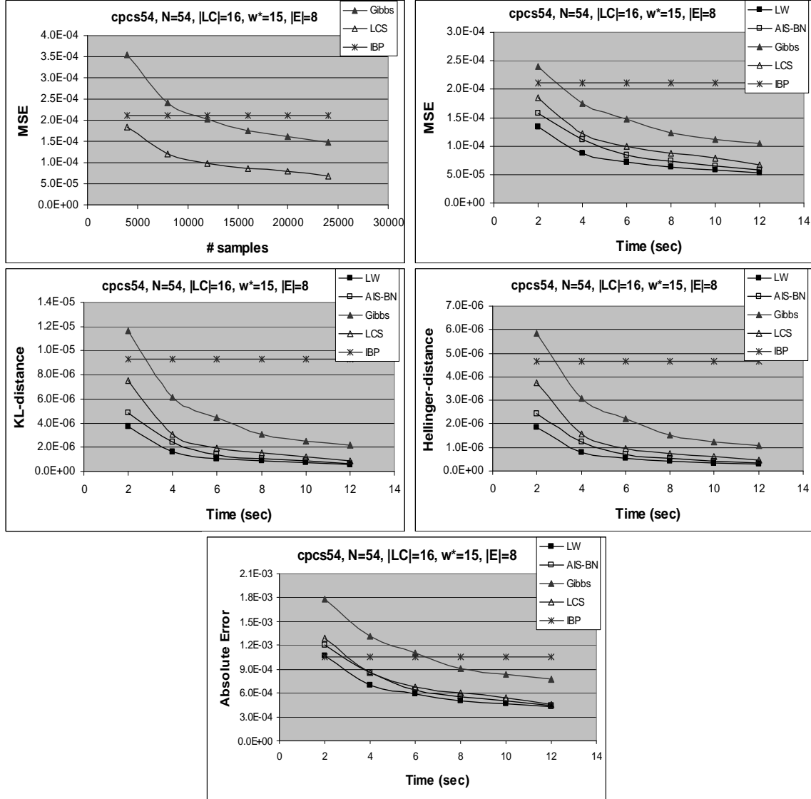
Figure 9: Comparing loop-cutset sampling (LCS), w_{LC}=5 , Gibbs sampling (Gibbs), likelihood weighting (LW), AIS-BN, and IBP on cpcs54 network, averaged over 20 instances, showing MSE as a function of the number of samples (top left) and time (top right) and KL-distance (middle left), squared Hellinger’s distance (middle right), and an average error (bottom) as a function of time.
