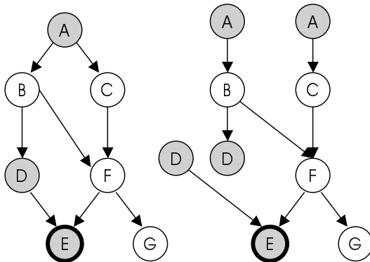
Figure 1: When nodes A and D in the loopy Bayesian network (left) are instantiated, the network can be transformed into an equivalent singly-connected network (right). In the transformation process, a replica of an observed node is created for each child node.
