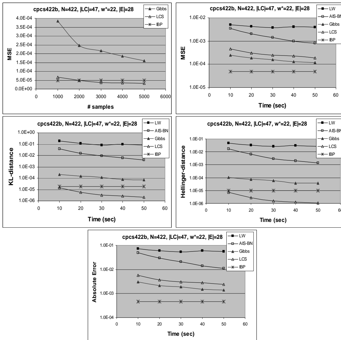
Figure 12: Comparing loop-cutset sampling (LCS), w_{LC}=14 , Gibbs sampling (Gibbs), likelihood weighting (LW), AIS-BN sampling, and IBP on cpcs422b network, averaged over 10 instances, showing MSE as a function of the number of samples (top left) and time (top right) and KL-distance (middle left), squared Hellinger's distance (middle right), and an average error (bottom) as a function of time.
