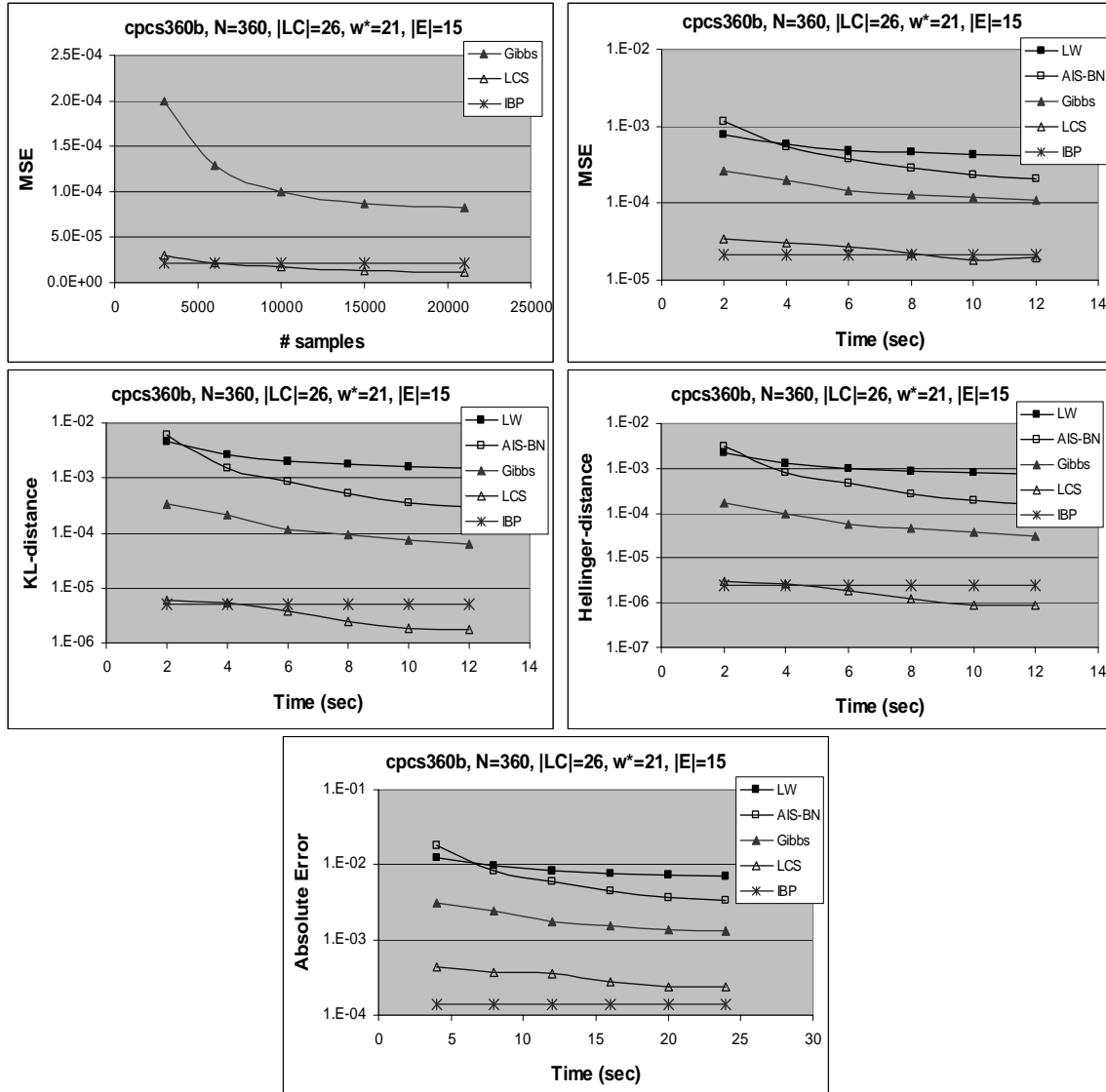
Figure 11: Comparing loop-cutset sampling (LCS), w_{LC}=3 , Gibbs sampling (Gibbs), likelihood weighting (LW), AIS-BN, and IBP on cpcs360b network, averaged over 20 instances, showing MSE as a function of the number of samples (top left) and time (top right) and KL-distance (middle left), squared Hellinger's distance (middle right), and an average error (bottom) as a function of time.
