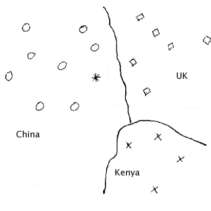
► Figure 14.1 Vector space classification into three classes.
