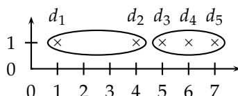
► Figure 17.7 Outliers in complete-link clustering. The five documents have the x -coordinates 1 + 2\epsilon, 4, 5 + 2\epsilon, 6 and 7 - \epsilon . Complete-link clustering creates the two clusters shown as ellipses. The most intuitive two-cluster clustering is \{\{d_1\}, \{d_2, d_3, d_4, d_5\}\} , but in complete-link clustering, the outlier d_1 splits \{d_2, d_3, d_4, d_5\} as shown.
