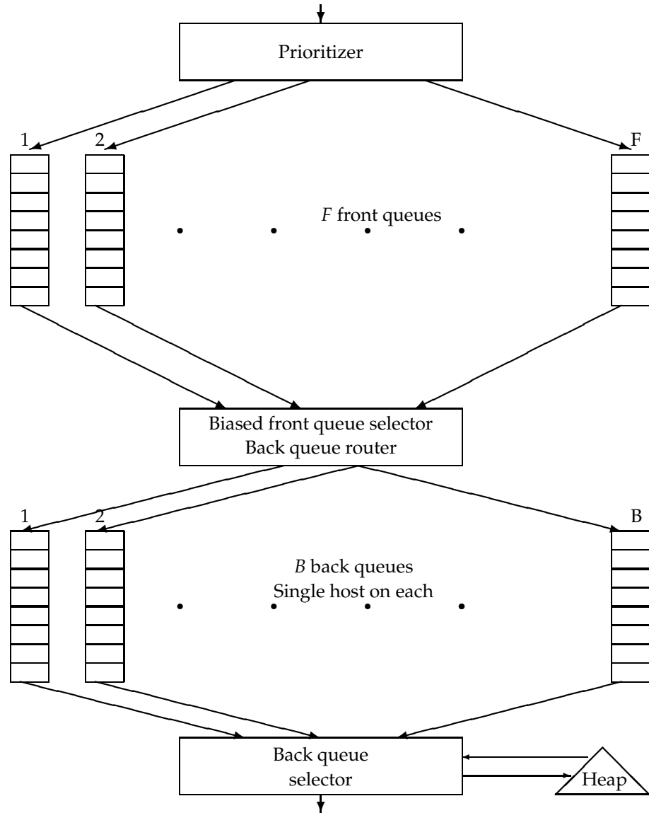
► Figure 20.3 The URL frontier. URL's extracted from already crawled pages flow in at the top of the figure. A crawl thread requesting a URL extracts it from the bottom of the figure. En route, a URL flows through one of several front queues that manage its priority for crawling, followed by one of several back queues that manage the crawler's politeness.
