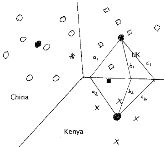
► Figure 14.3 Rocchio classification.
