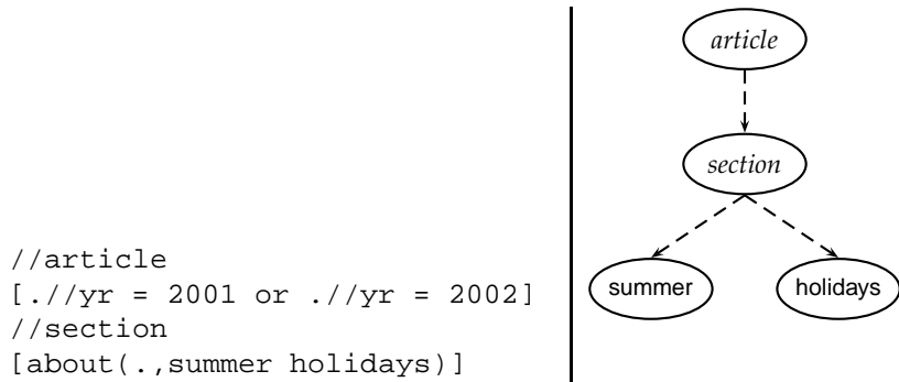
► Figure 10.3 An XML query in NEXI format and its partial representation as a tree.
