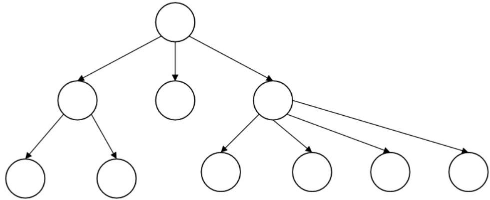
► Figure 3.2 A B-tree. In this example every internal node has between 2 and 4 children.
