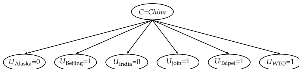
► Figure 13.5 The Bernoulli Naive Bayes model.
