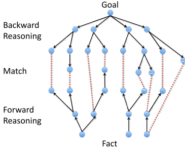
Fig. 4. Matching between Goals and Facts Fig. 5. Example of Distributed Execution
