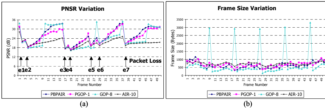
Figure 6. Comparison between PBPAIR and existing techniques, where PLR is assumed to be 10%: (a) PSNR variation (b) frame size variation (image source: FOREMAN.QCIF, 300 frames)
