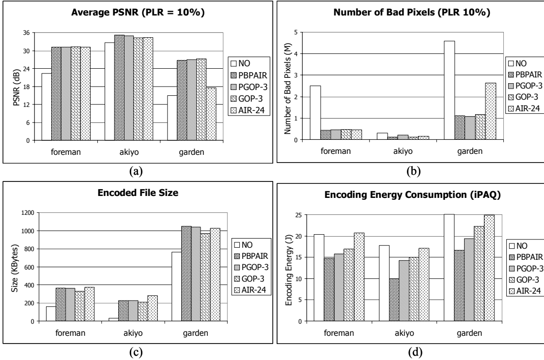
Figure 5. Comparison between PBPAIR and existing techniques, where PLR is assumed to be 10%: (a) the average PSNR (b) the number of bad pixels as an image quality measure (c) the encoded file size (d) the encoding energy consumption using iPAQ as a performance measure (image sources: FOREMAN.QCIF, AKIYO.QCIF, and GARDEN.QCIF, 300 frames)
