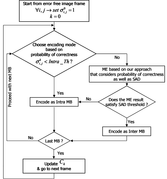
Figure 2. PBPAIR error resilient coding
