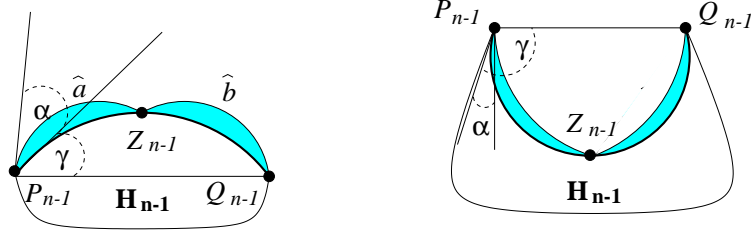
Fig. 3. Arcs \hat{a} and \hat{b} pass through P_{n-1}, Z_{n-1} and Q_{n-1}, Z_{n-1} respectively. Their tangents form an angle \alpha with the tangents of P_{n-1}Z_{n-1} and Q_{n-1}Z_{n-1} . The shape of the region bounded by \hat{a} and P_{n-1}Z_{n-1} depends on the concavity/convexity of P_{n-1}Q_{n-1} and \alpha .
