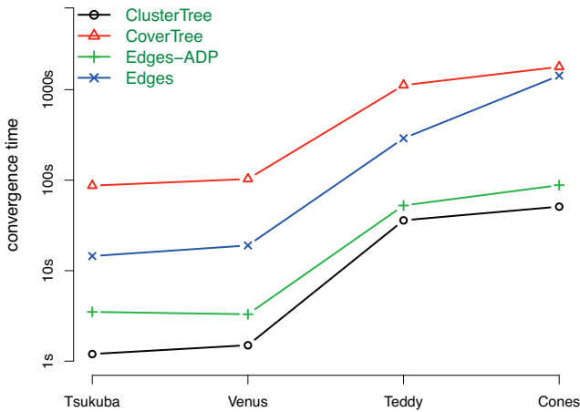
Figure 7: For images from the Middlebury dataset, our algorithm is about twice as fast as Edges-ADP.
