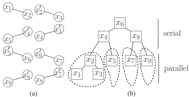
Figure 3: (a) Dual-decomposition using independent edges is highly parallelizable but slow to converge. (b) The cluster tree is also easily parallelizable, but since the underlying model is a covering tree, convergence is not compromised.
