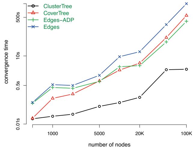
Figure 6: For randomly generated graphs, our algorithm achieves a significant speedup as the model size increases.
