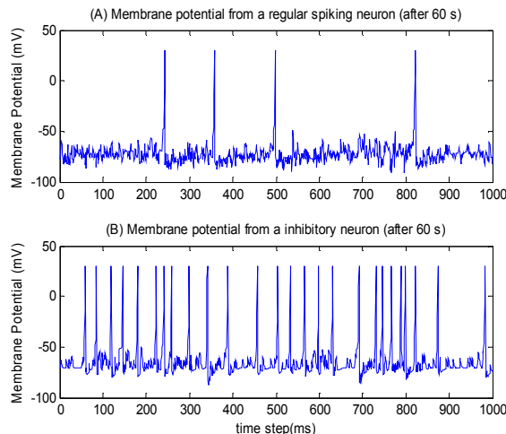
Figure 2: Membrane potential produced by Izhikevich neurons: (a) Regular Spiking Neuron (b) Inhibitory Neuron.
