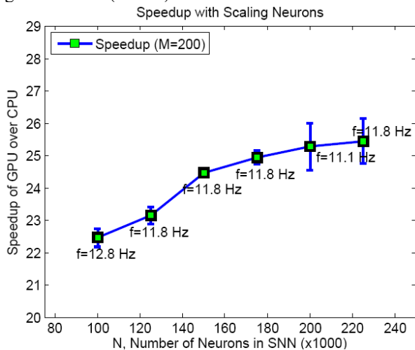
Figure 9: Speedup of GPU with respect to a single CPU for different network size ( N ) and different synaptic connections per neuron ( M ). Simulations were run 5 times with different random number seed. The notation f=n Hz denotes the mean firing rate of 5 simulations. Error bar denotes the standard deviation of the speedup.
