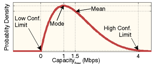
Figure 4. Probability distribution.
