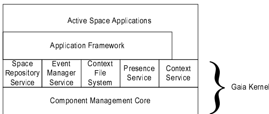
Figure 7: Architecture of the Gaia system
